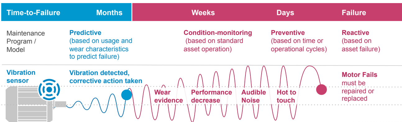
Figure 1: PdM Motor vibration analysis example
